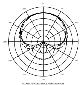
Polar Pattern
